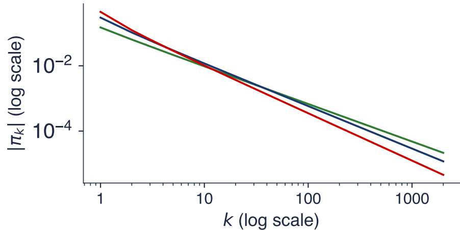
Slow decay: |\pi_k| \sim k^{-d-1}/|\Gamma(-d)|
