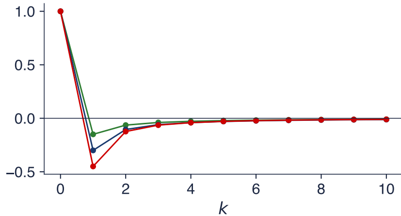
Weights \pi_0, \dots, \pi_{10} of (1 - L)^d
