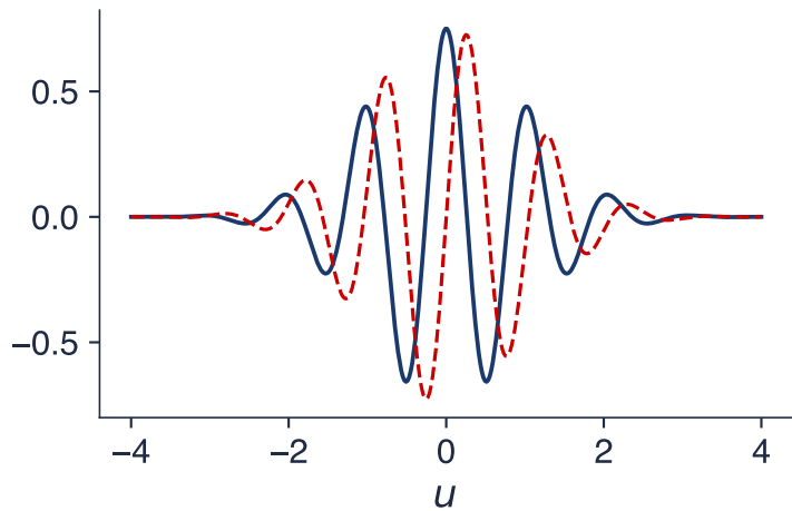
Morlet \psi(u) , \omega_0 = 6
