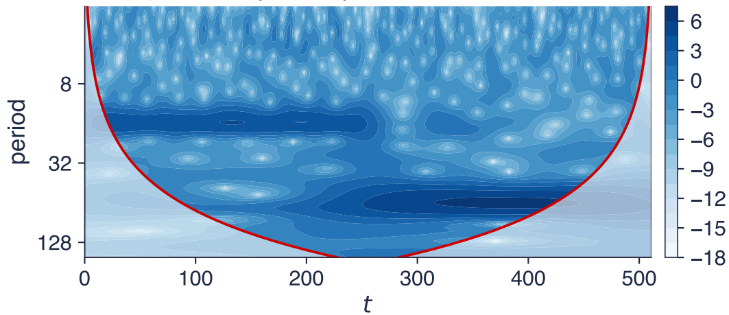
Scalogram \log_2 |W(s, t)|^2 : period 16, then 64
