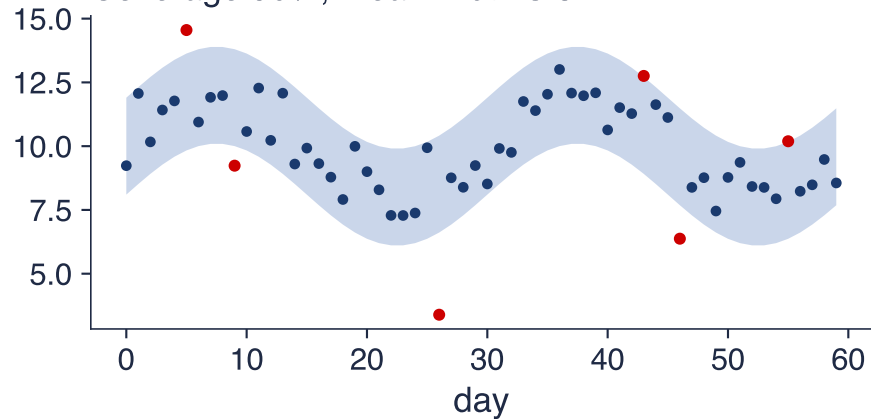
Coverage 90%, mean width 3.8
