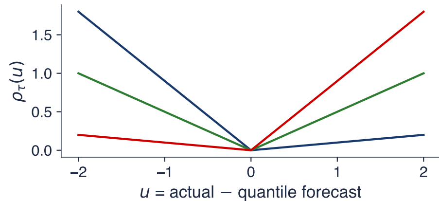
Pinball loss
