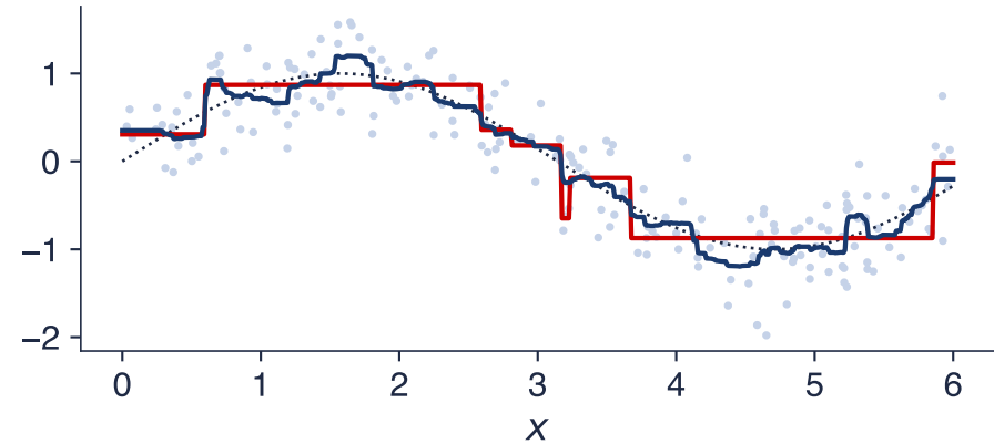
Piecewise constant fits
