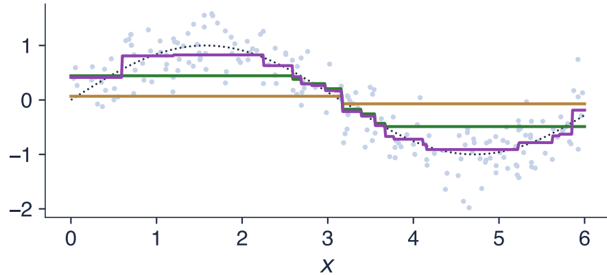
Boosting with stumps, \nu = 0.1
