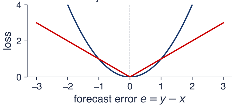
Symmetric losses
