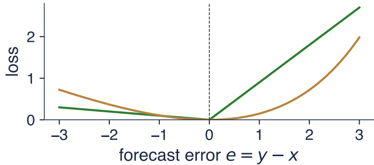
Asymmetric losses
