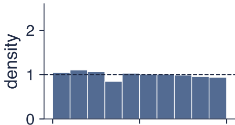
calibrated: N(0, 1)
