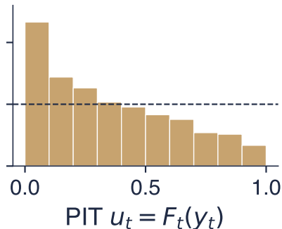
biased: N(0.5, 1)
