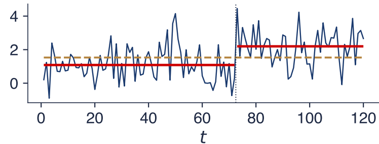
A mean shift after T_1 = 72
