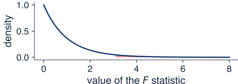
Reference distribution of the Chow test
