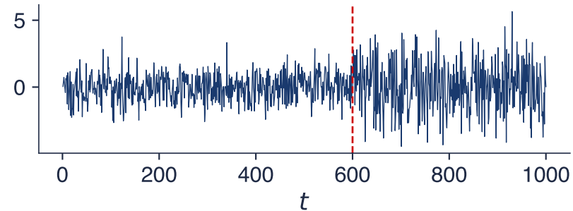
Standard deviation 1, then 1.8
