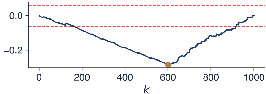
Centred cumulative sum of squares
