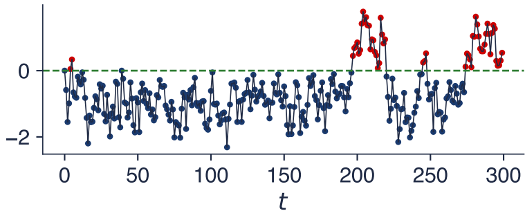
Simulated SETAR path
