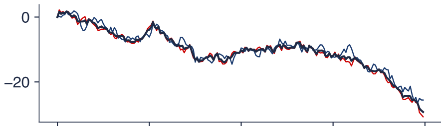
Levels and the common trend
