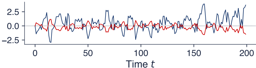
Transitory parts: stationary
