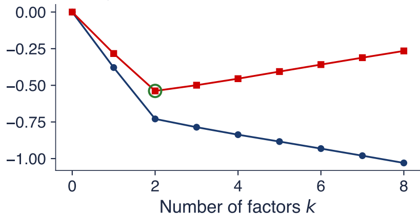
Penalty per factor 0.096
