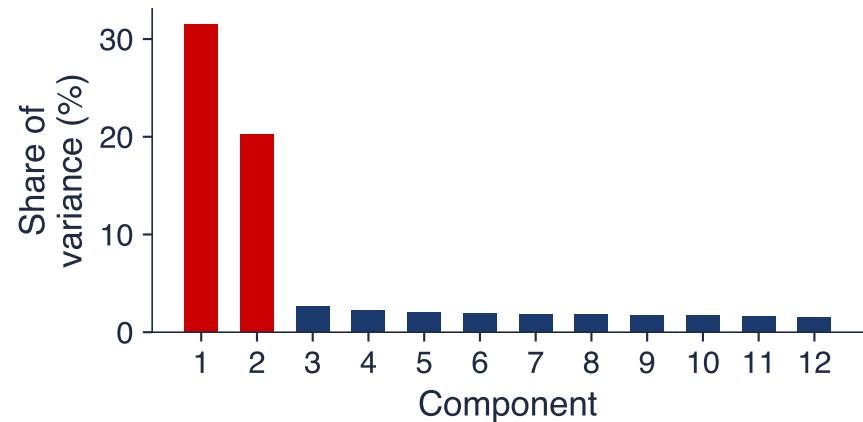
Scree plot (2 true factors)
