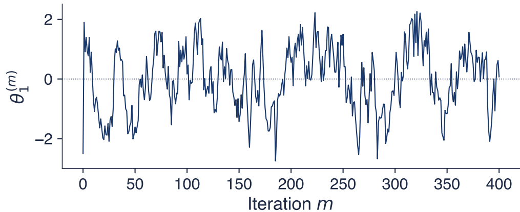
Trace plot
