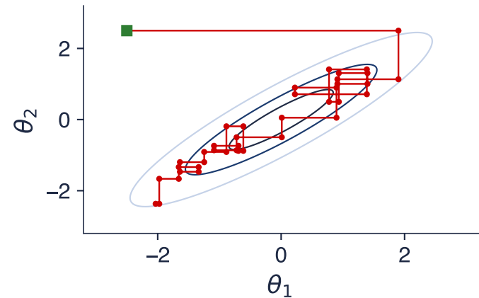
Target: correlation 0.9
