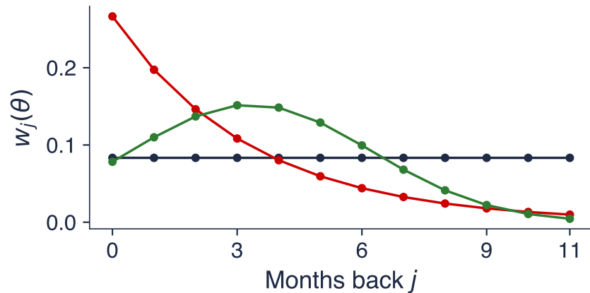
Exponential Almon, K = 12
