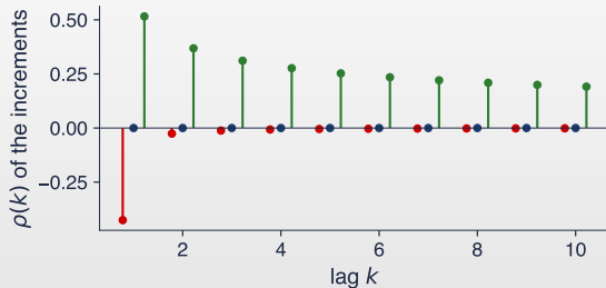
Fractional Gaussian noise
