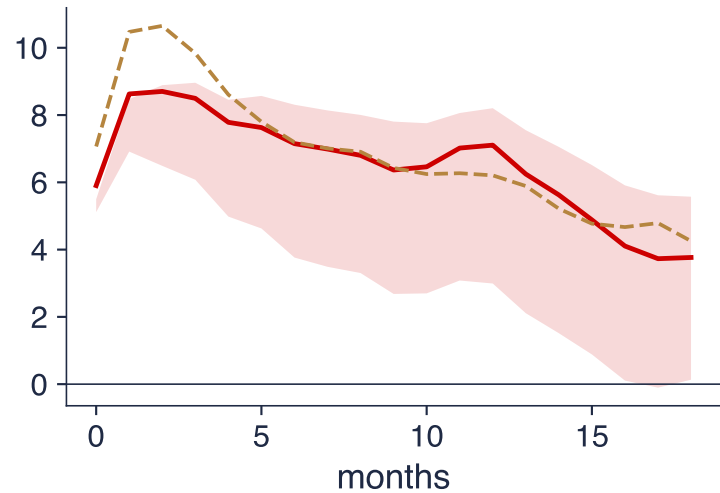
Oil-specific demand shock
