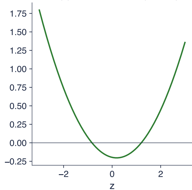
\tau(z) = \tau_1 z + \tau_2 (z^2 - 1)
