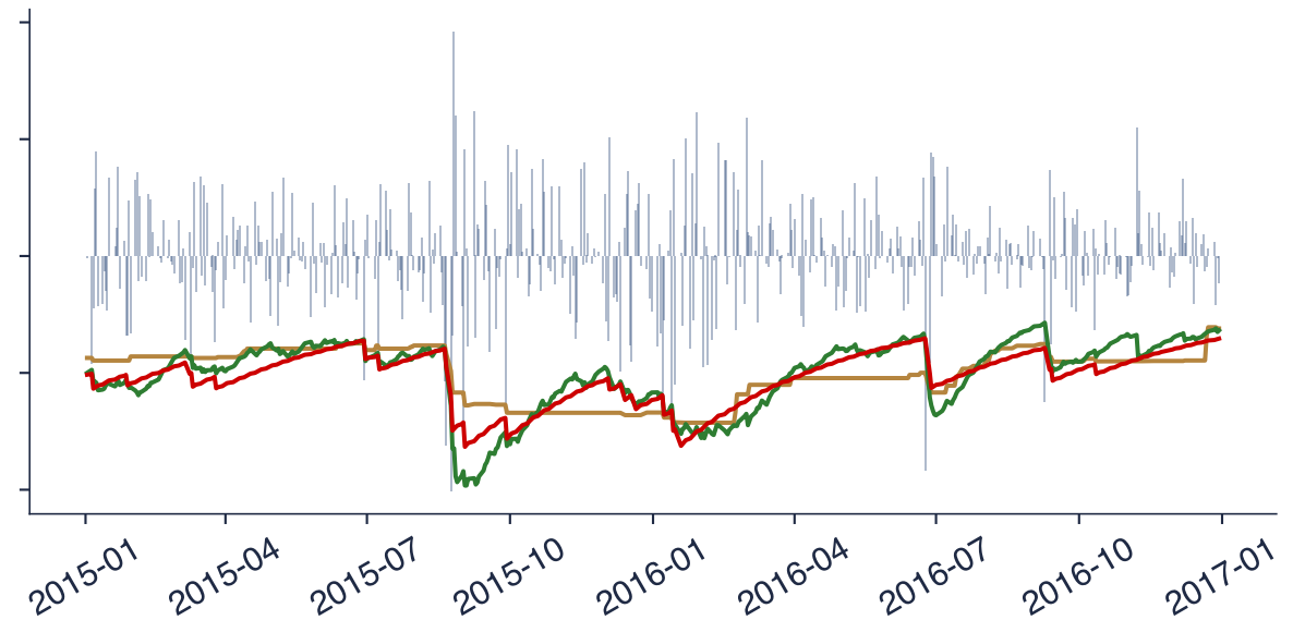
ES 5% (tail mean)
