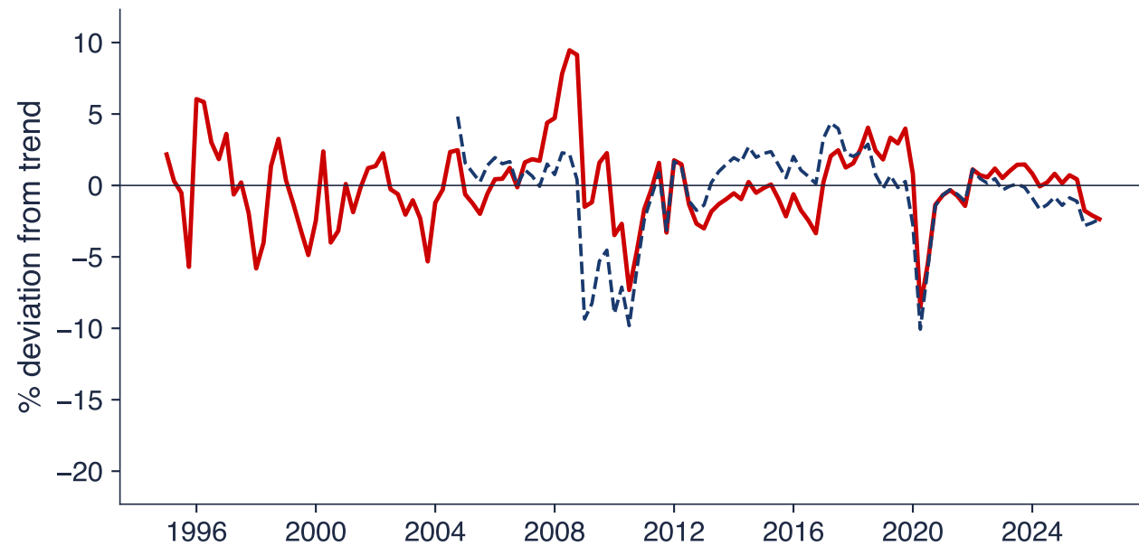
HP filter, \lambda = 1600
