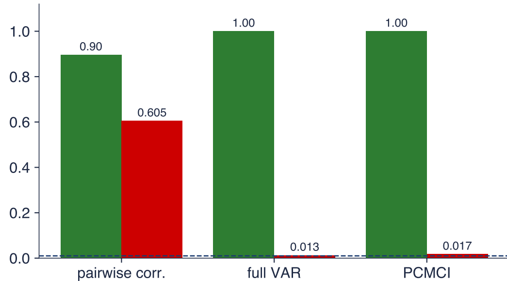
6 variables, T = 500
