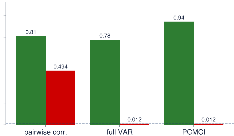
20 variables, T = 150
