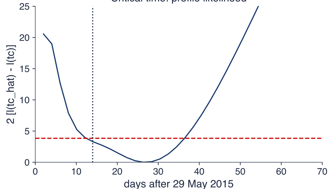
Critical time: profile likelihood
