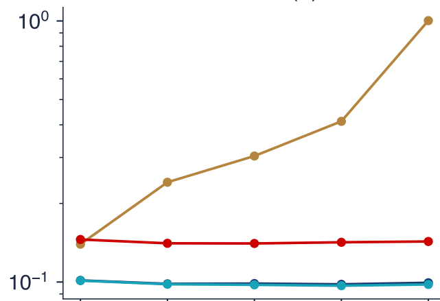
DGP: MA(1)
