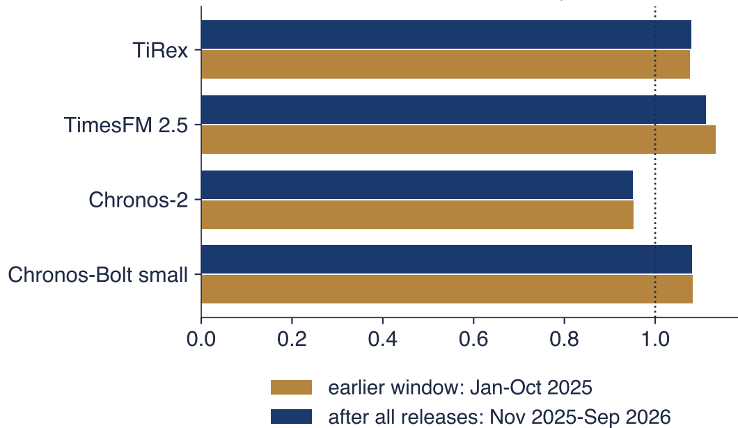
Romanian load: MAE / expert ARX
