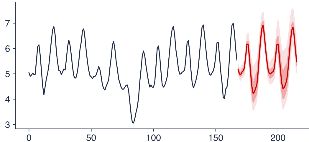
Romanian load (GW), hourly
