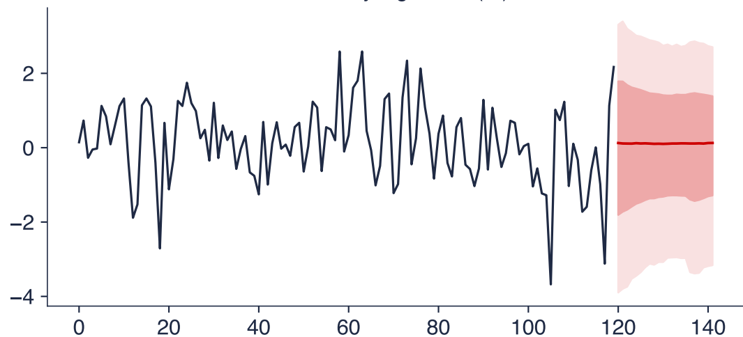
BET daily log return (%)
