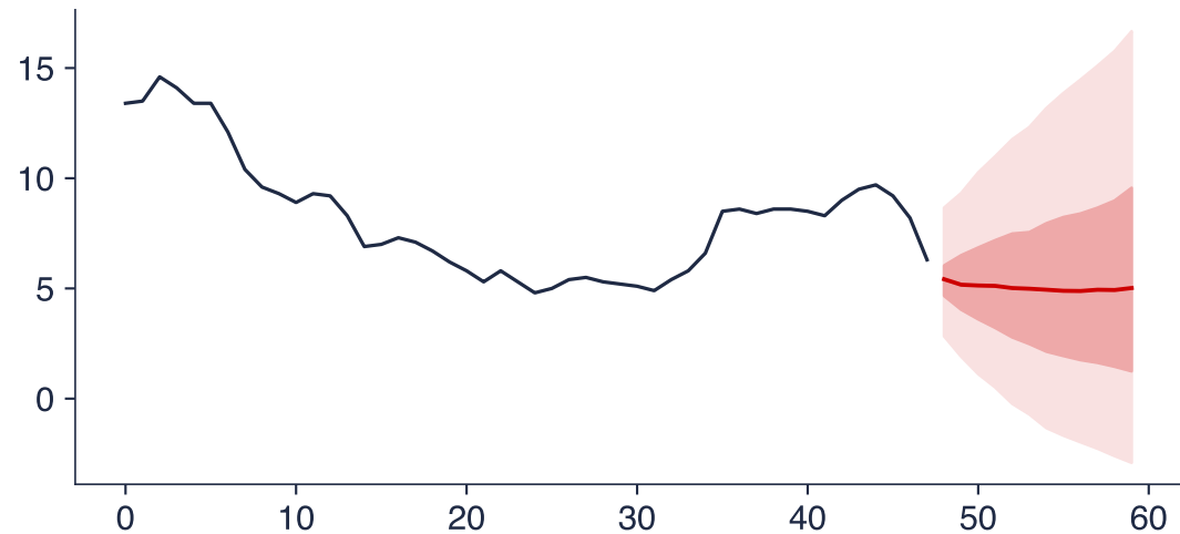
Romanian HICP inflation (%), monthly
