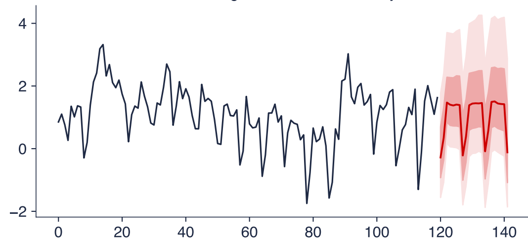
Bitcoin log realised variance, daily
