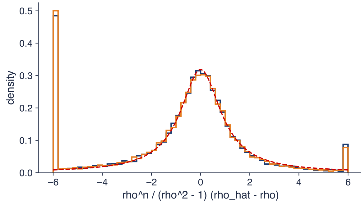
mildly explosive: \rho = 1 + 1/n^{0.7} = 1.0245 , n = 200
