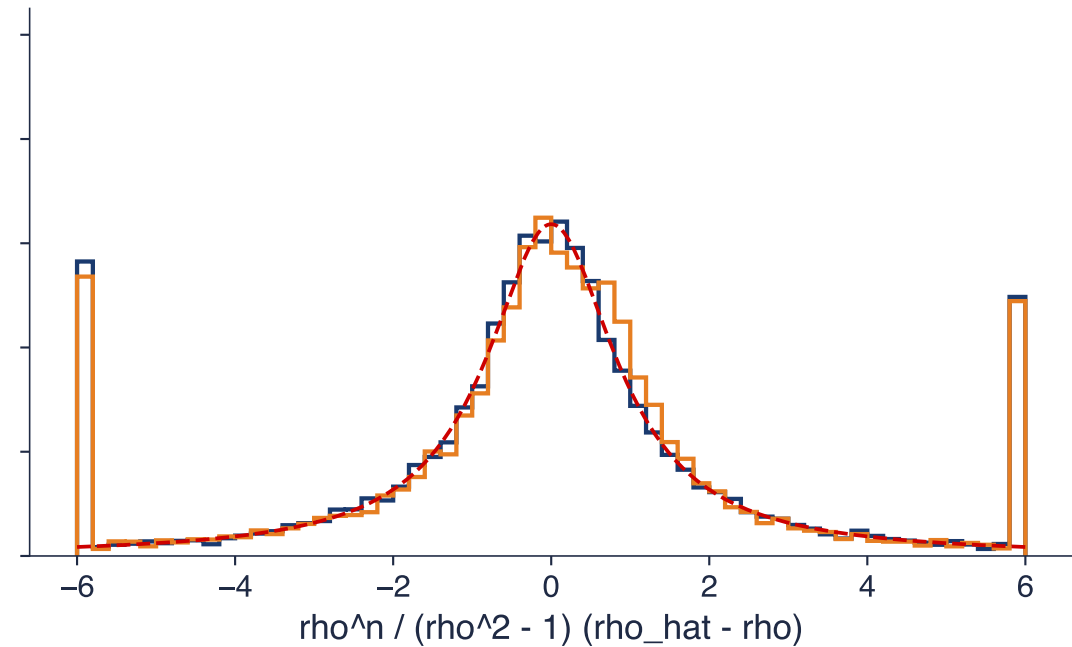
fixed explosive: \rho = 2 , n = 30
