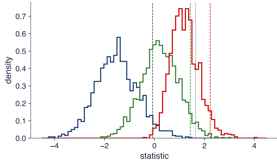
Null distributions, T = 400 (dashed: 95% quantiles)
