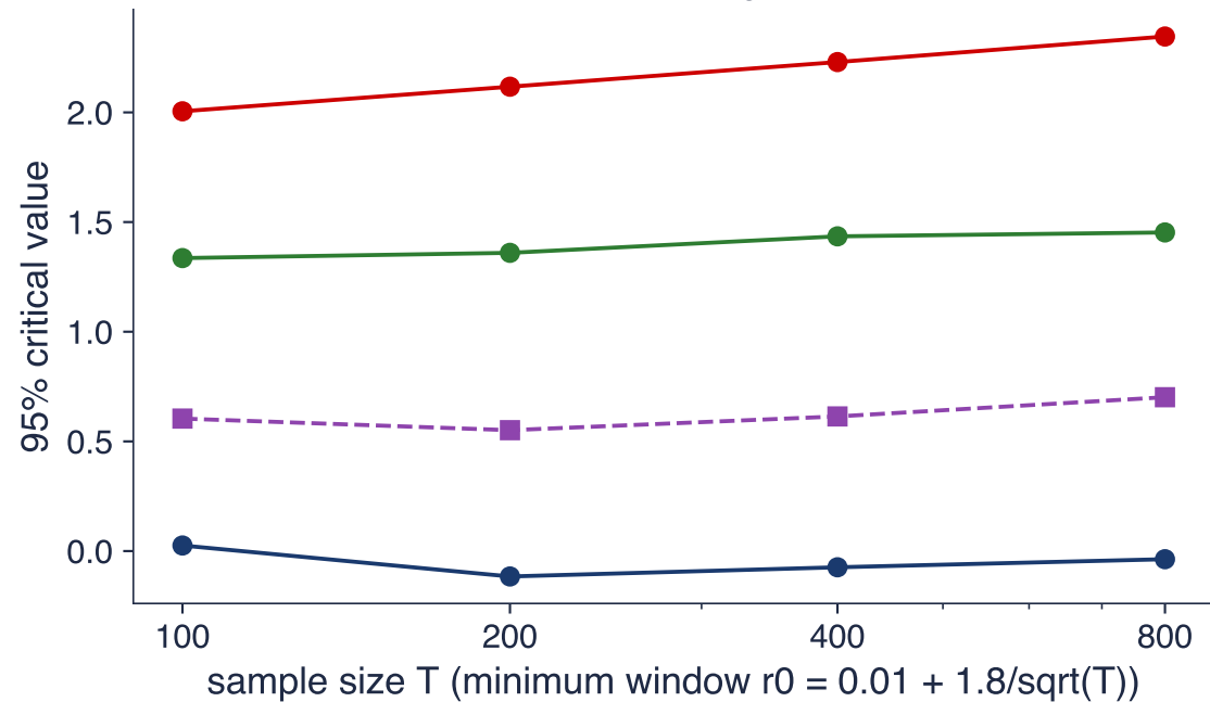
Critical values against T
