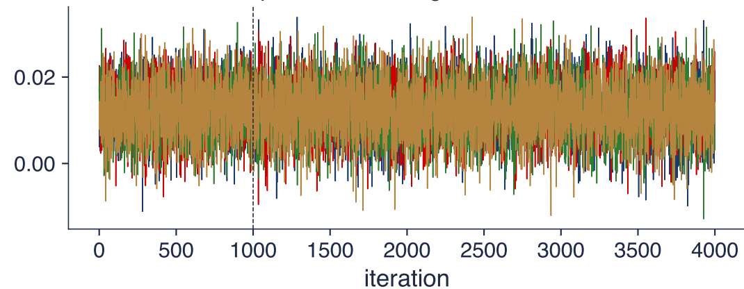
Slope b, centred regressor: traces
