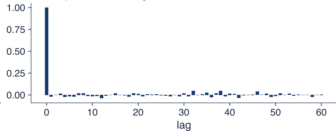
Slope b, centred regressor: autocorrelation of the draws
