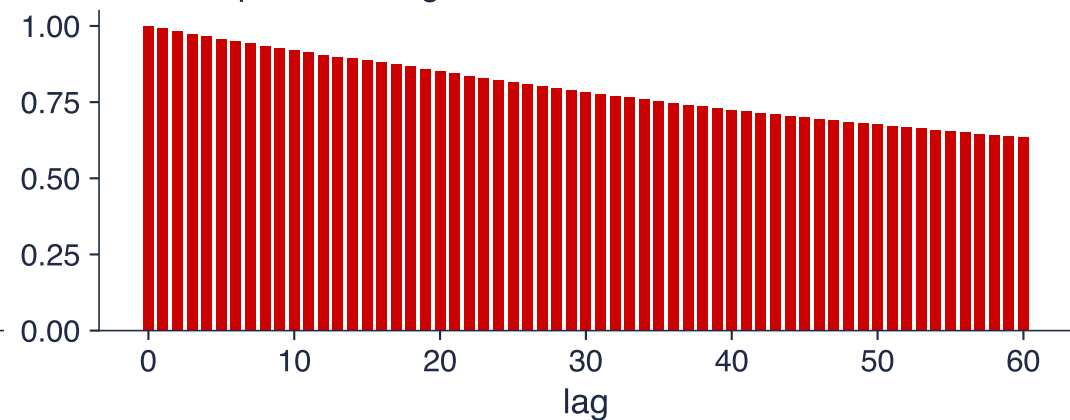
Slope b, raw regressor: autocorrelation of the draws
