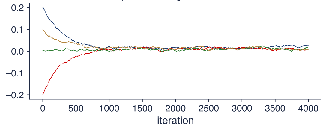
Slope b, raw regressor: traces
