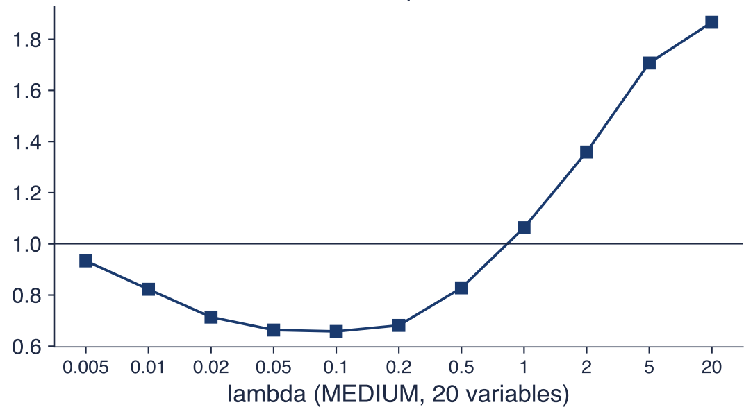
Out-of-sample MSFE
