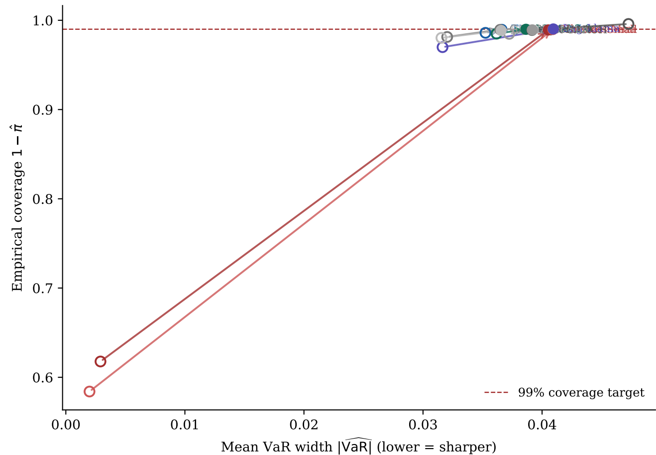
Calibration--Efficiency Frontier (all nine forecasters, \alpha = 0.01 )
