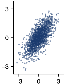
Gaussian \rho = 0.71
