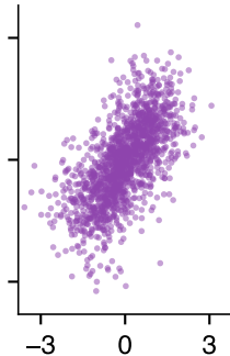
Frank \theta = 5.74
