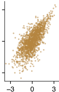
Gumbel \theta = 2.00
