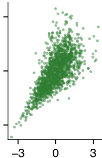
Clayton \theta = 2.00
