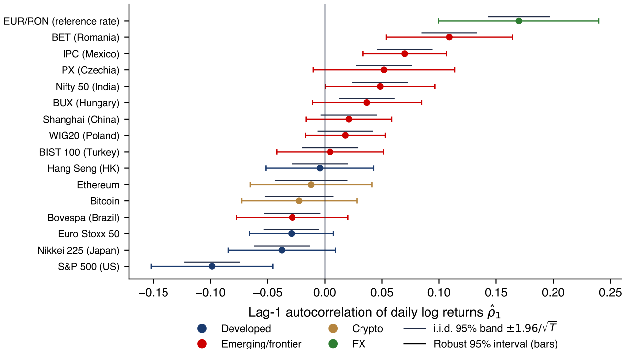
Lag-1 autocorrelation across markets (full samples)
