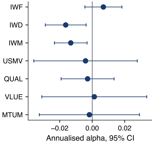
FF5 + momentum alpha
