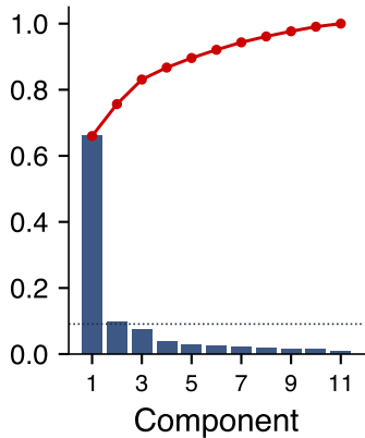
Scree plot
