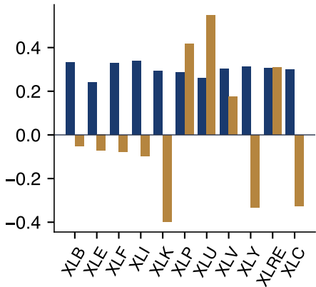
Eigenvector loadings
