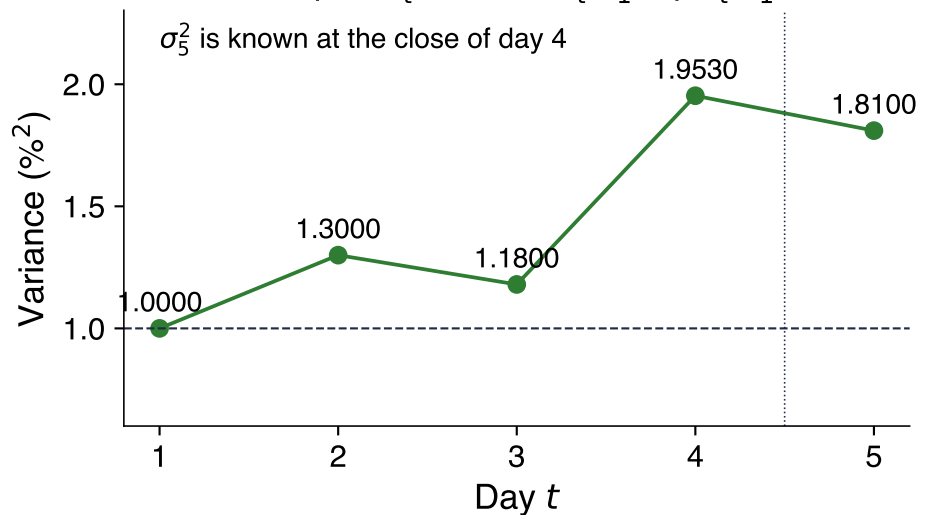
Output: \sigma_t^2 = \omega + \alpha \varepsilon_{t-1}^2 + \beta \sigma_{t-1}^2
