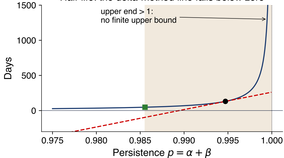
Half-life: the delta-method line falls below zero
