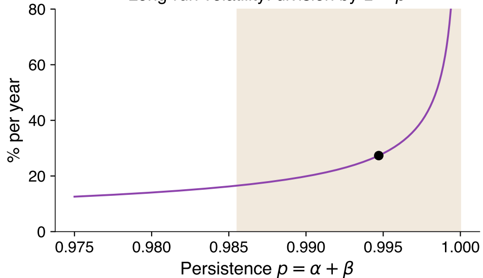
Long-run volatility: division by 1 - p
