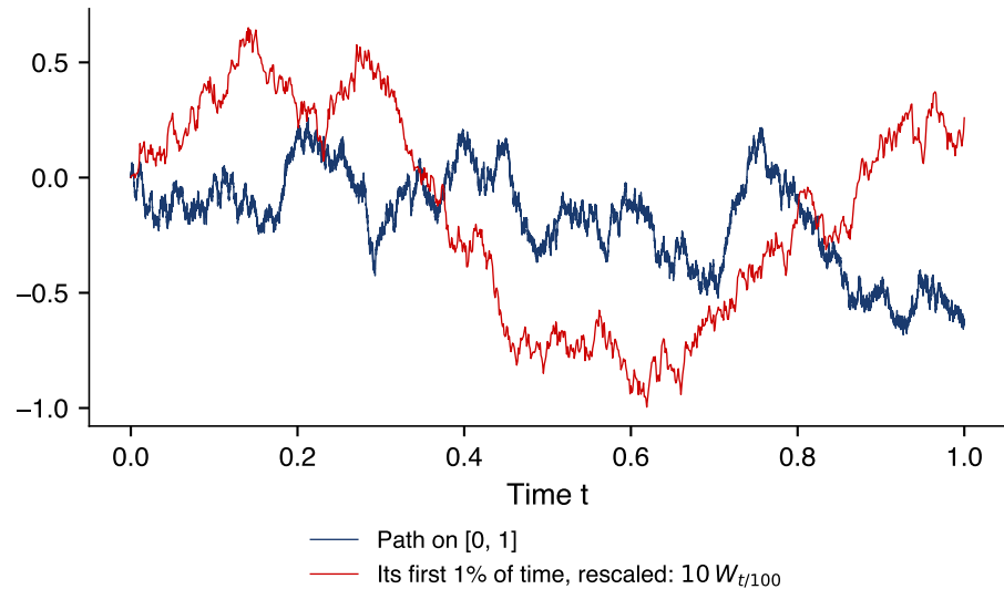
Self-similarity: zoom in and the path looks the same
