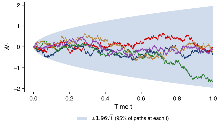
Five Brownian paths on [0, 1]
