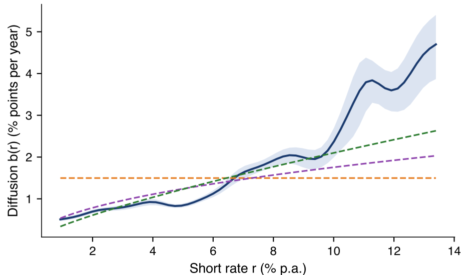
Diffusion: estimated precisely
