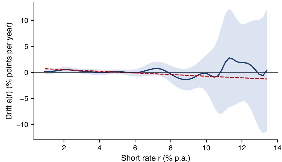
Drift: estimated imprecisely
