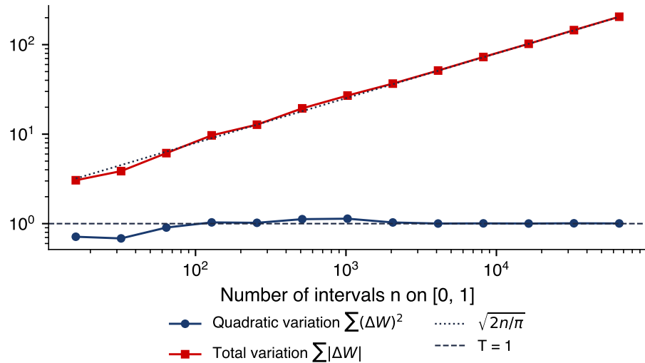
One Brownian path, finer and finer grids
