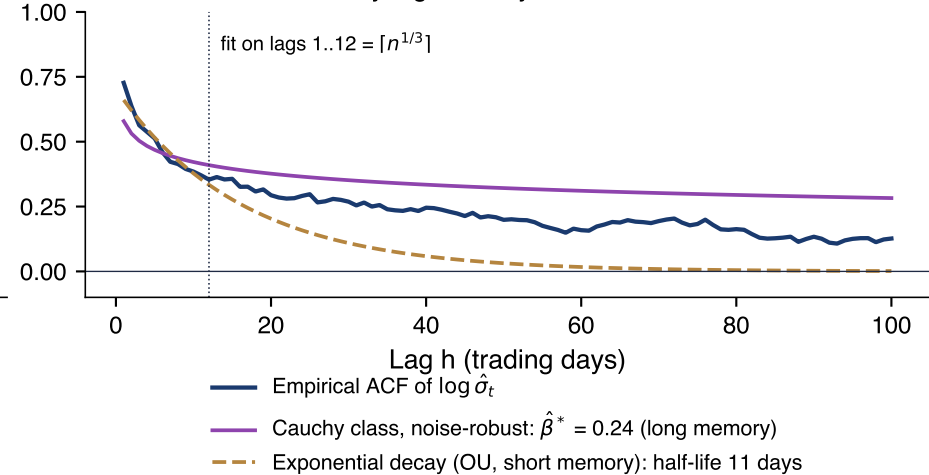
Persistence: ACF of daily log-volatility
