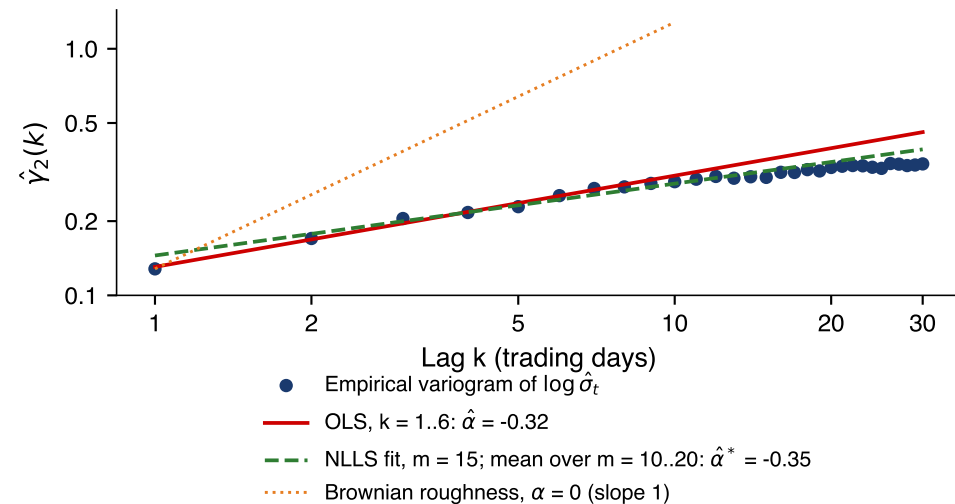
Roughness: variogram of daily log-volatility (log-log)
