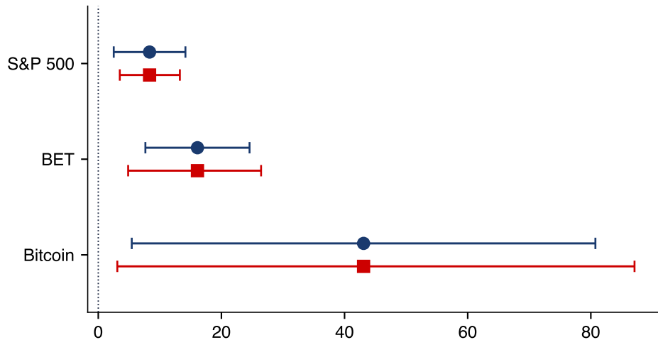
Log drift m (% per year), 95% interval
