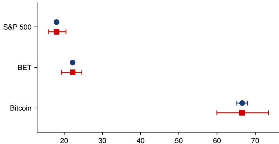
Volatility \sigma (% per year), 95% interval
