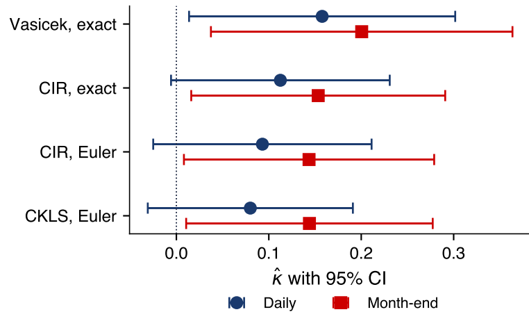
Mean-reversion speed
