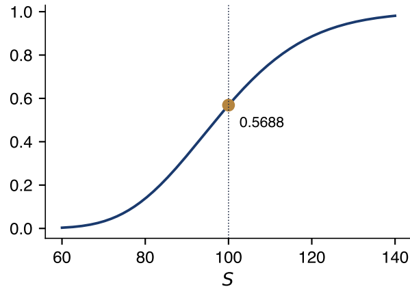
Delta \Phi(d_1)
