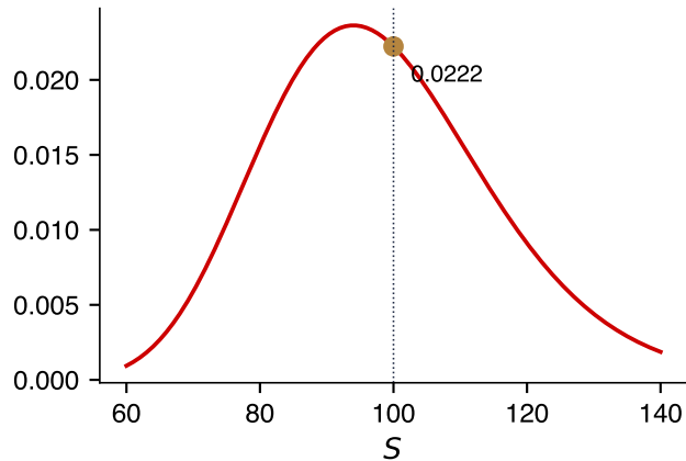
Gamma \phi(d_1)/(S\sigma\sqrt{\tau})
