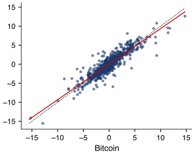
Daily returns (%)
