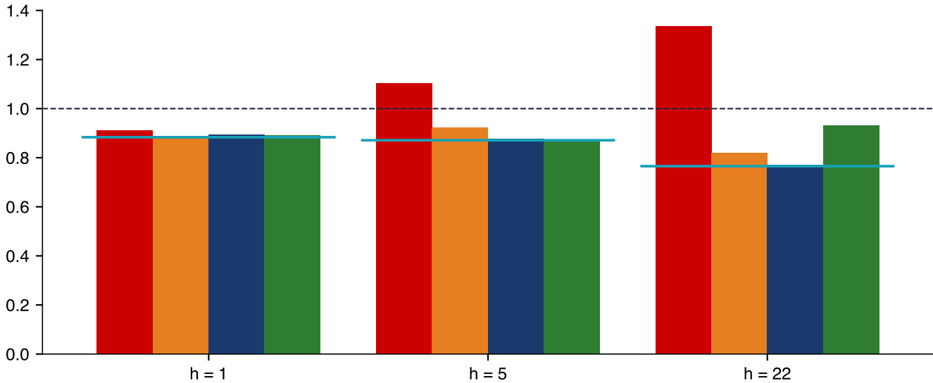
Sig-LK: QLIKE relative to HAR (mean over 50 assets)
