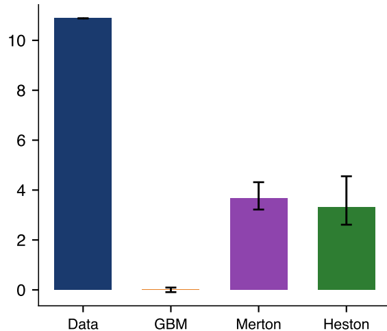
Excess kurtosis
