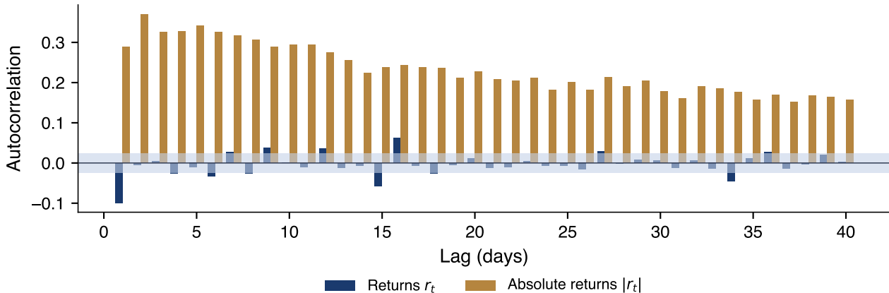
S&P 500 2000-2026: direction is almost unpredictable, risk is predictable
