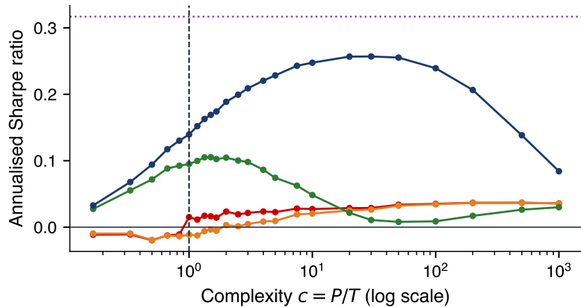
Sharpe ratio of the timing strategy
