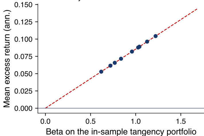
Exact: every sector on the line
