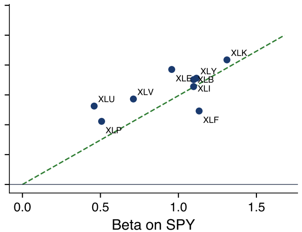
SPY is not the tangency portfolio
