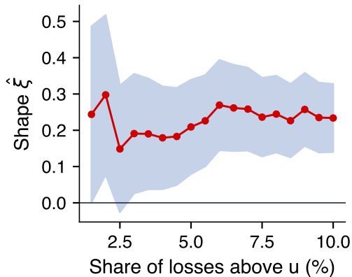
Stability of \xi across thresholds
