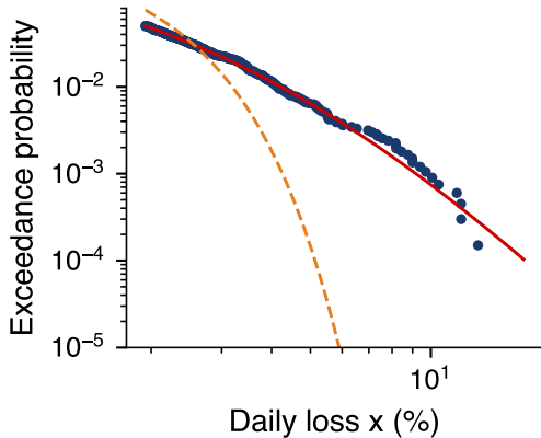
BET: largest 5% of daily losses
