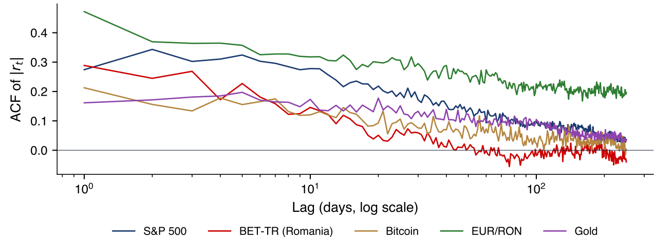
Volatility clustering and long memory: slow, hyperbolic-like decay
