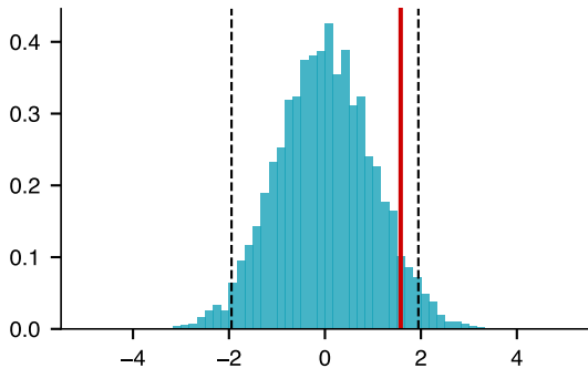
HRP minus GMV, block 1: p = 0.12
